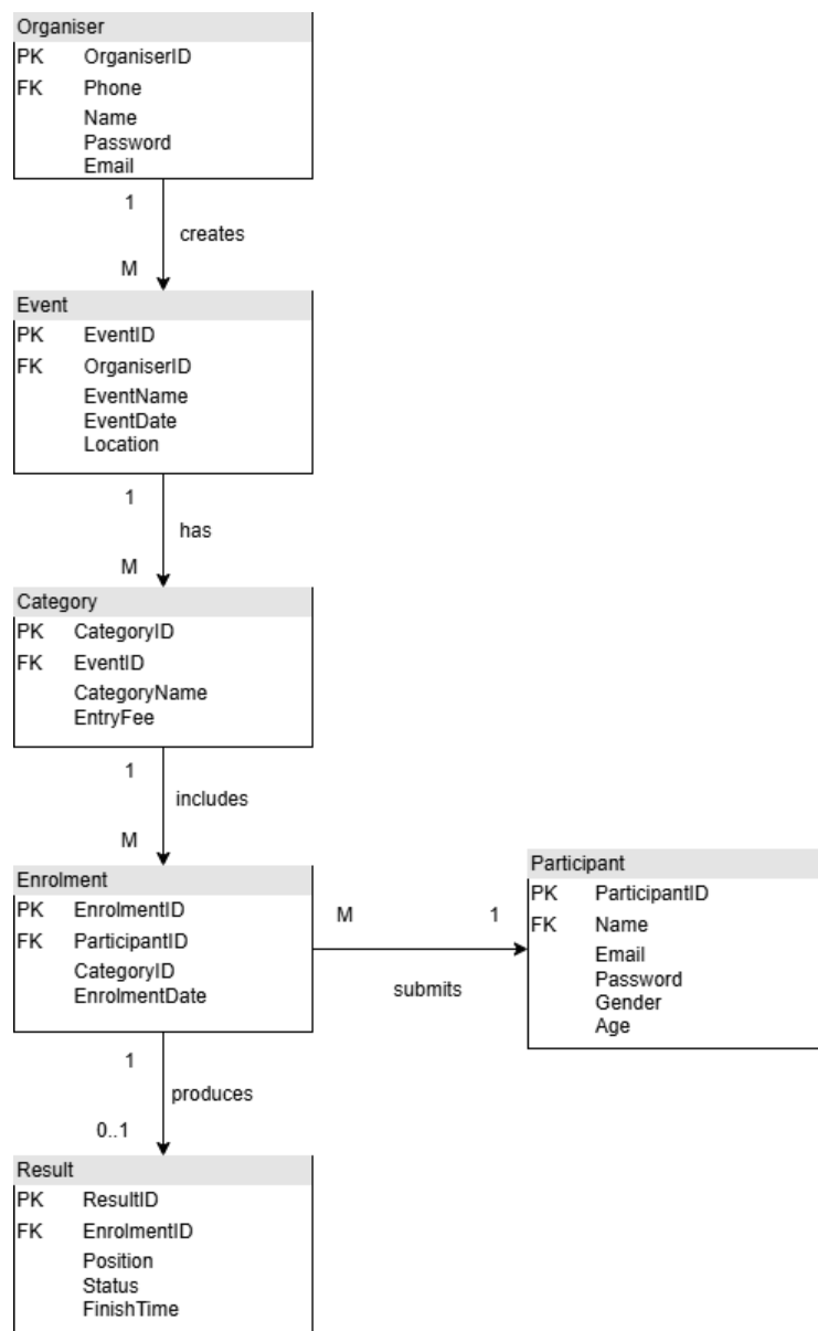
ERD with 6 entities containing cardinalities for every relationship
